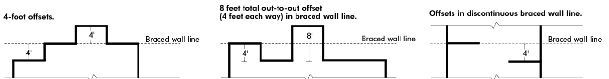
FIGURE 21.25-C PERMITTED OFFSETS
